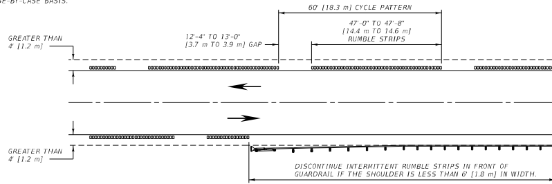
INTERMITTENT RUMBLE STRIP SPACING
