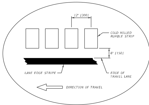
TYPICAL SHOULDER INSTALLATION (ASPHALT PAVEMENT)
