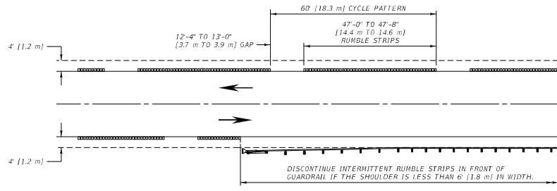
INTERMITTENT RUMBLE STRIP SPACING
