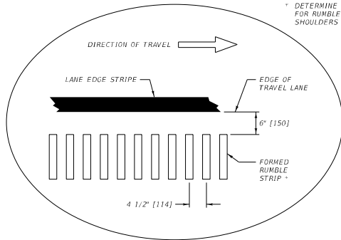
TYPICAL SHOULDER INSTALLATION (CONCRETE PAVEMENT)
