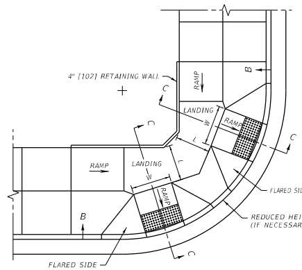
COMBINED (PARALLEL / PERPENDICULAR) CURB RAMP
