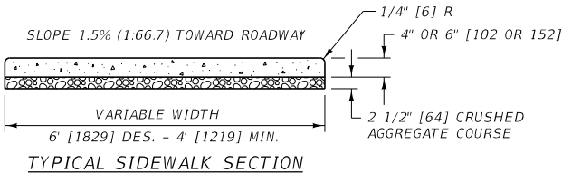
TYPICAL SIDEWALK SECTION
