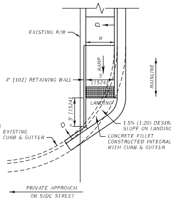
CURB RAMP OPTIONS FOR PRIVATE APPROACH OR SIDE STREETS WITH CURB RETURNS BUT WITHOUT SIDEWALK
