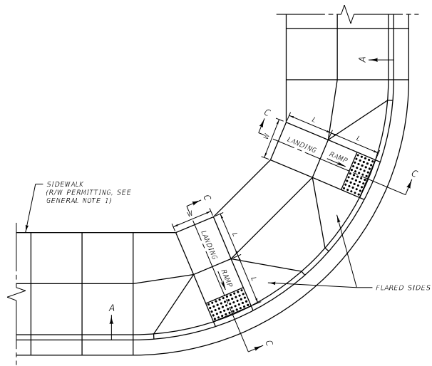
PERPENDICULAR CURB RAMP
