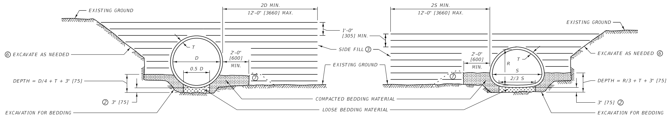
1-STANDARD BEDDING INSTALLATION
