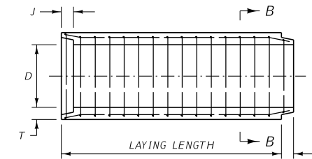
TYPICAL LONGITUDINAL SECTION
