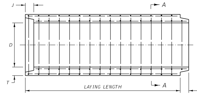
TYPICAL LONGITUDINAL SECTION
