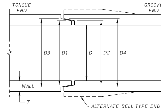
JOINT DETAIL
