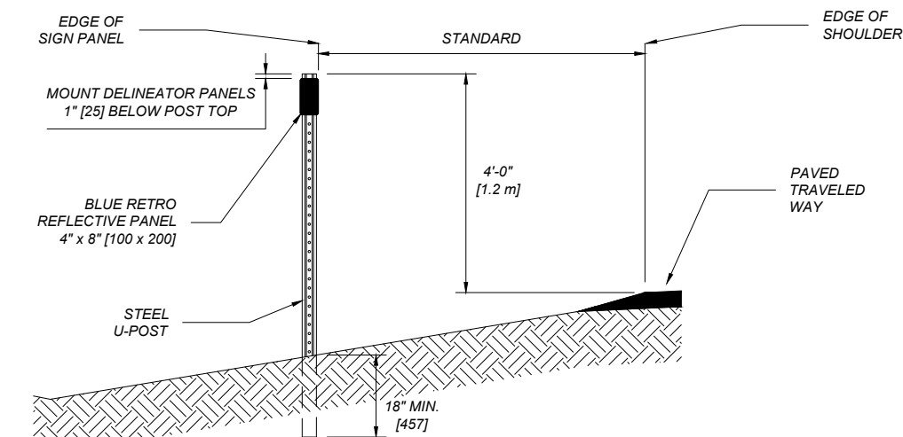
① DETAIL A
