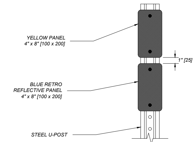
① DETAIL A
