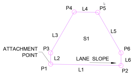
Figure 5: 4" Curb Diagram
