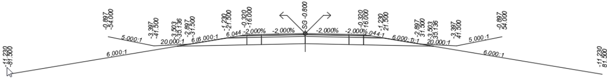
Rural Undivided 2 Lane – GDS 2.4 / RDM 5-19 12' Lanes, 4' Shoulder, Rural Slope Table
