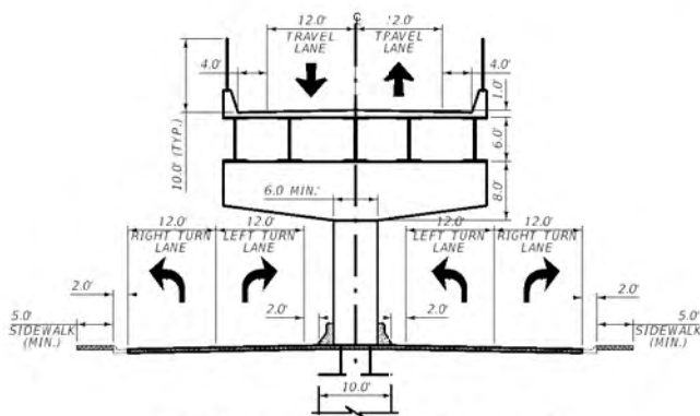
27TH ST TYPICAL SECTION
