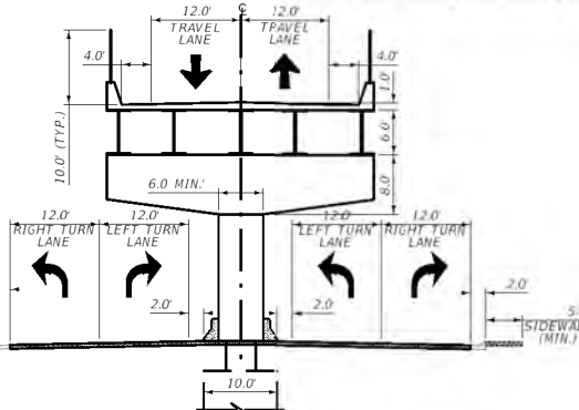
27TH ST TYPICAL SECTION
