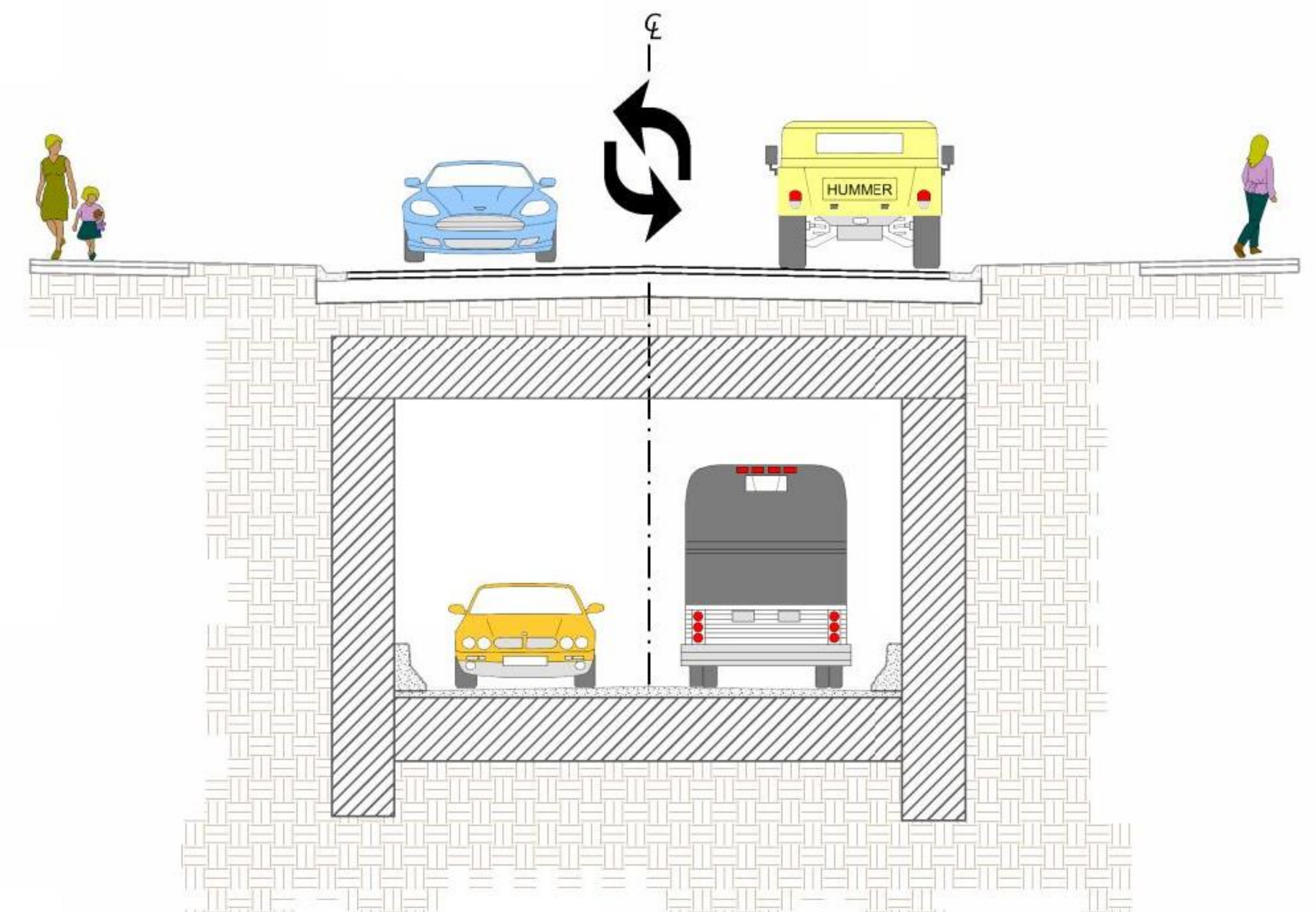
2-Lane Tunnel
