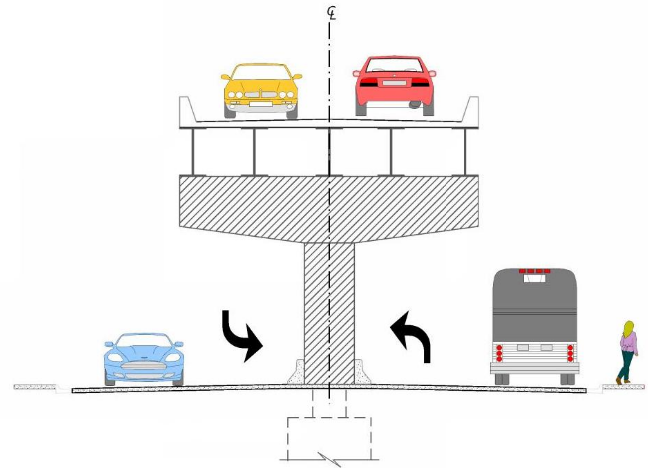
2-Lane Overpass
