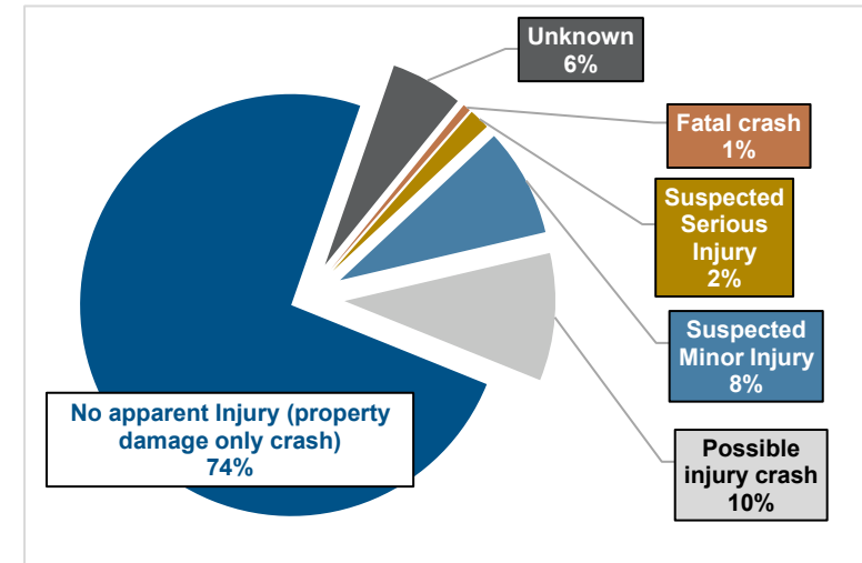
Figure 20: Crash Severity
