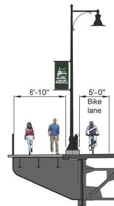
INWARD MOUNTED LIGHTPOLE - BIKE LANE OPTION
