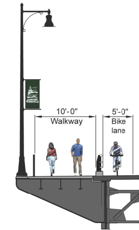
OUTWARD MOUNTED LIGHTPOLE - BIKE LANE OPTION
