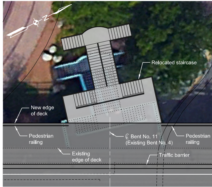
RELOCATE EXISTING STAIRCASE
