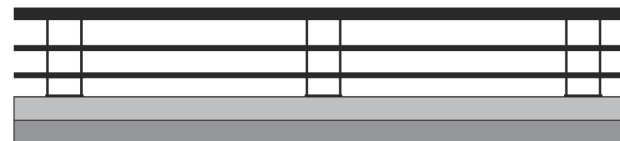
TRAFFIC RAIL OPTION 2: 42" TALL STEEL RAIL
