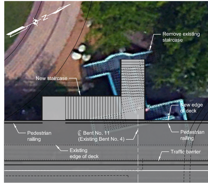
REPLACE EXISTING STAIRCASE
