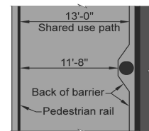
INWARD MOUNTED LIGHTPOLE - SHARED USE PATH OPTION
