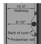
INWARD MOUNTED LIGHTPOLE - BIKE LANE OPTION
