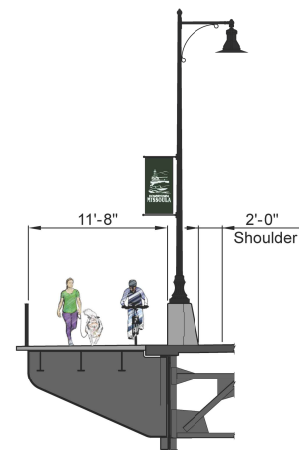
INWARD MOUNTED LIGHTPOLE - SHARED USE PATH OPTION
