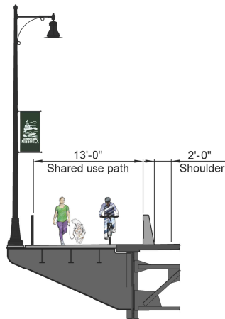
OUTWARD MOUNTED LIGHTPOLE - SHARED USE PATH OPTION
